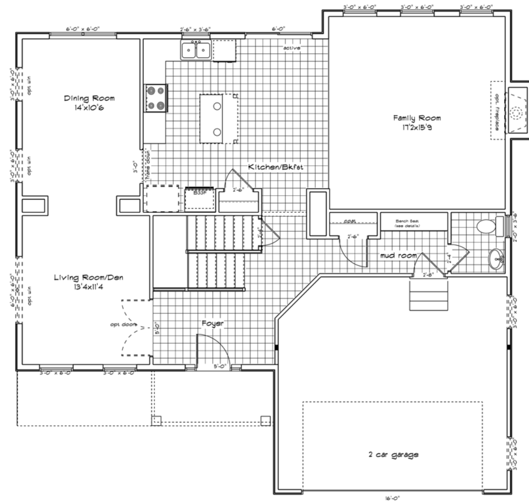
First Floor
